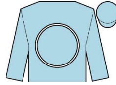
CYCLONITE
